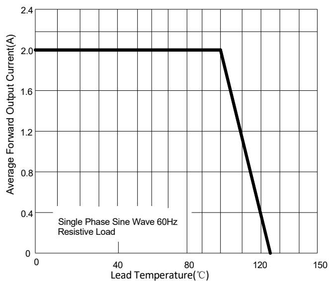
FIG1: Io-TL Curve
